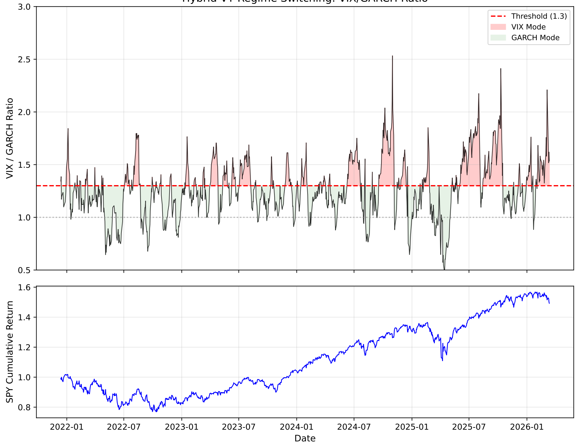
Hybrid VT Regime Switching: VIX/GARCH Ratio
