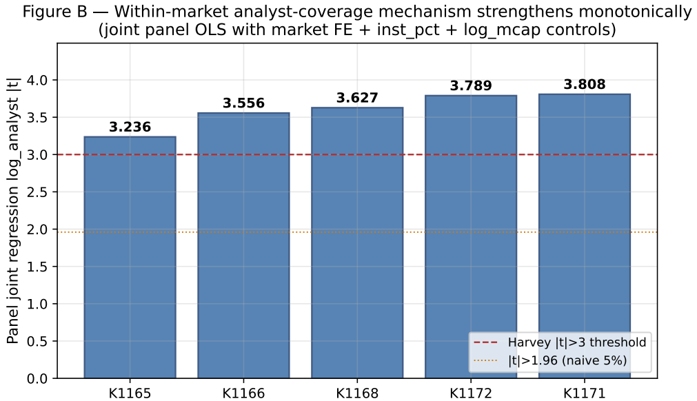
Figure 2: Panel joint log(analyst) t -statistic trajectory (3.236 → 3.808) across five N-extension iterations (K1165, K1166, K1168, K1172, K1171). The horizontal dashed line marks the Harvey–Liu–Zhu (2016) |t| = 3.0 threshold; all five iterations exceed it.
