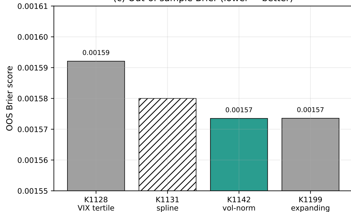
(c) Out-of-sample Brier (lower = better)
