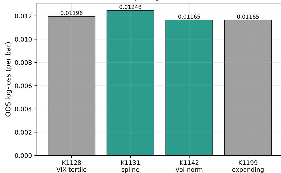
(b) Out-of-sample log-loss (lower = better)
