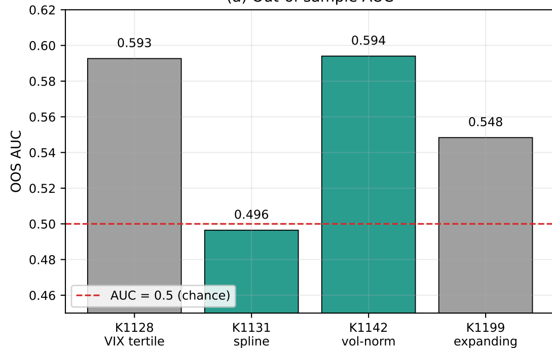
(a) Out-of-sample AUC
