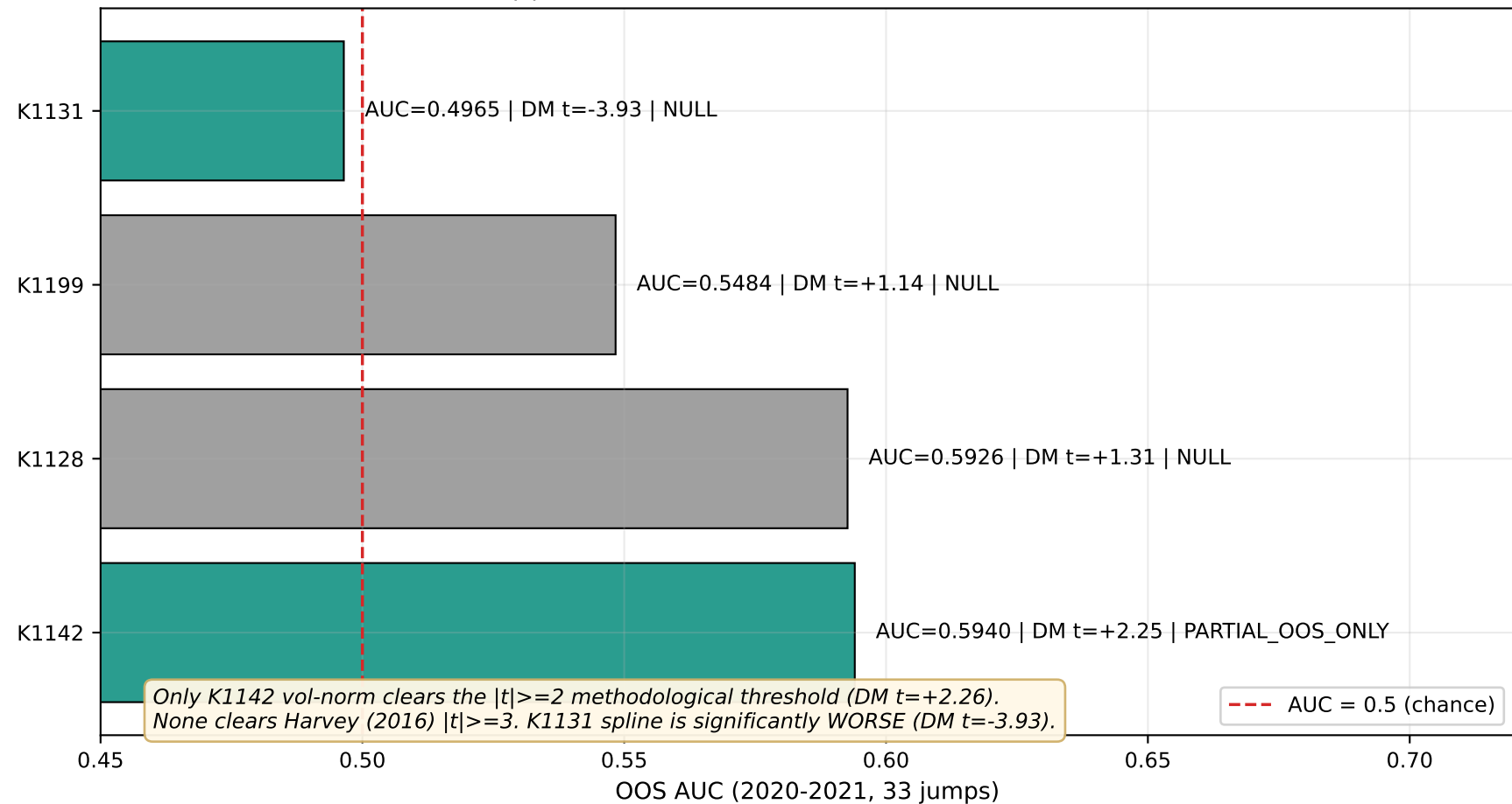
K1205 Fig. C | OOS AUC ranking across K1128 4-branch experiments Green = DM |t| \geq 2 (methodological threshold); Gray = not significant
