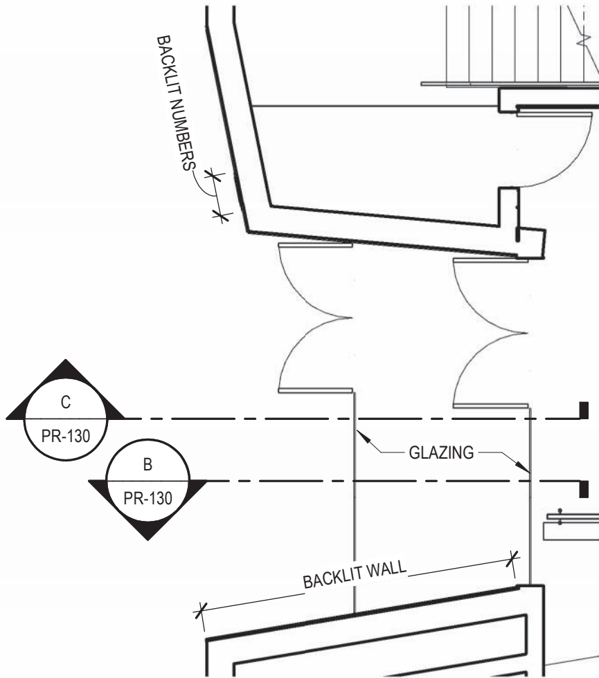
A PLAN
