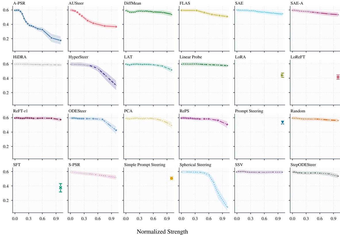
SuperGLUE MultiRC ↑
