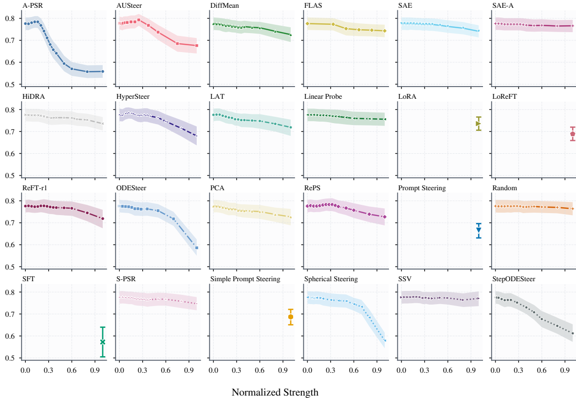
SuperGLUE RTE \uparrow
