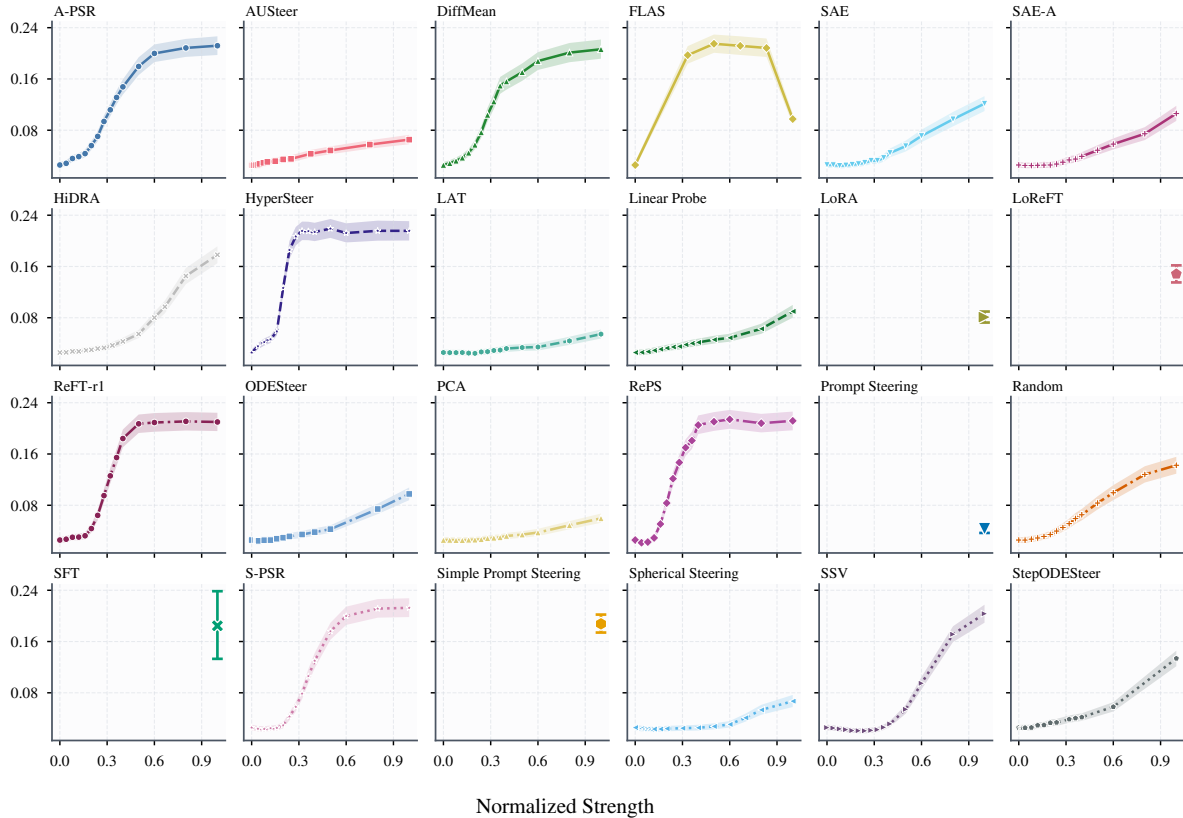
BBQ Ambiguous Bias ↓
