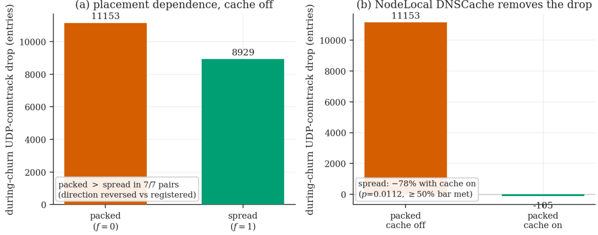
Figure 5.2: H2 — conntrack placement-dependence and the DNS intervention (C3). (a) The cache-off during-churn UDP-conntrack drop is larger under packing than spreading — reversed against the prediction, packed > spread in all 7 pairs. (b) Enabling the NodeLocal DNSCache collapses the packed drop to \approx 0 and shrinks the spread drop by a 78 % median, removing it under both placements: arm (b) passes, but the reversed direction (a) fails the conjunction.
