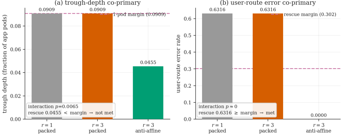
Figure 5.3: H3 — replication rescue under node-drain (C2) , across the three cells. (a) Trough depth: the anti-affine rescue (0.0455) falls below the one-pod margin (0.0909, dashed), which the r=1 and r=3 -packed cells sit on by construction — the depth face cannot adjudicate. (b) User-route error: anti-affine r=3 fully rescues ( 0.632 \rightarrow 0 ), clearing the 0.302 margin. The conjunction fails only on the depth co-primary it could not test.
