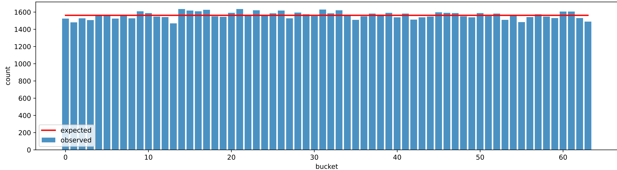
Bucketed test | NIST-III, N bits=769, samples=100000, buckets=64, chi2=65.124, p-value=0.4027
