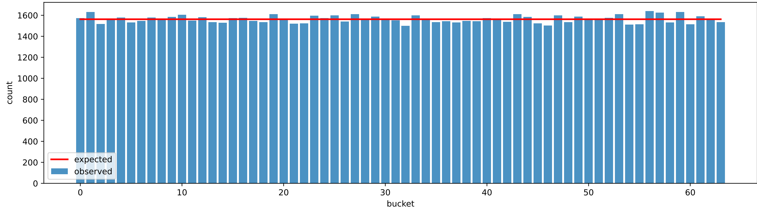
Bucketed test | NIST-I, N bits=513, samples=100000, buckets=64, chi2=46.538, p-value=0.9403
