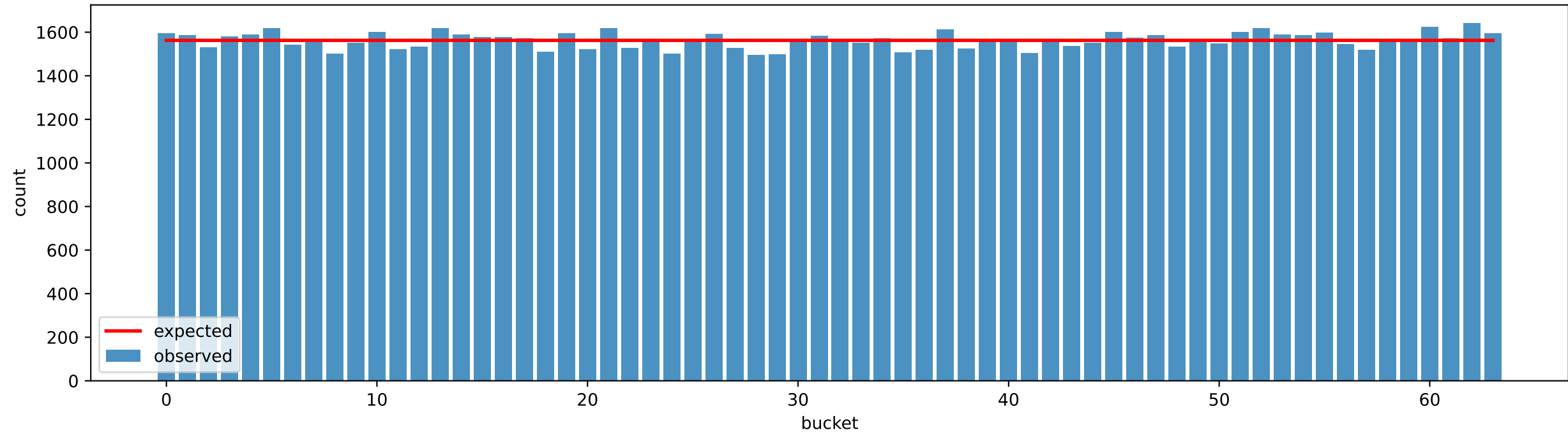
Bucketed test | NIST-V, N bits=1025, samples=100000, buckets=64, chi2=52.604, p-value=0.8218
