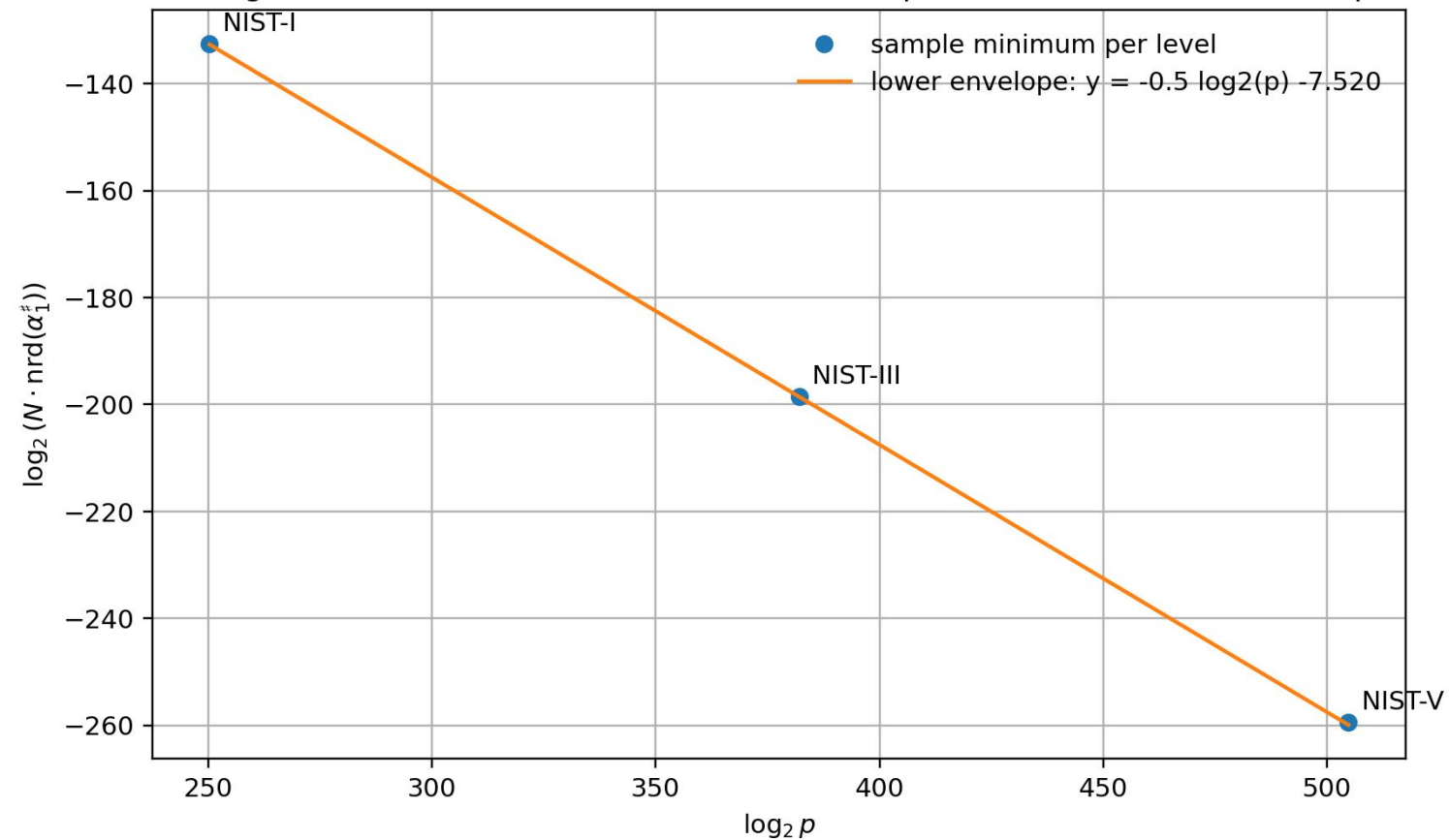
SQLsign trace-dual shortest reduced norm: sample minima and lower envelope
