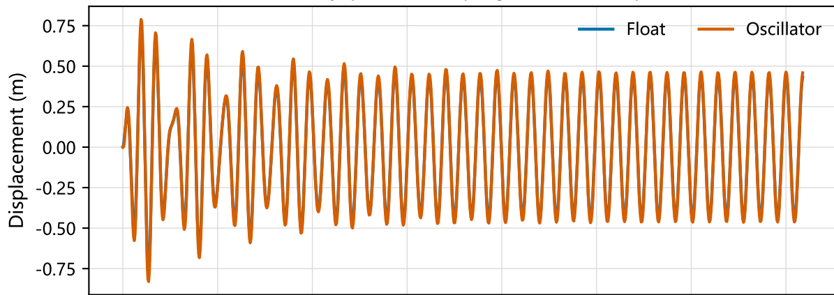
Q1 velocity-power-damping transient response
