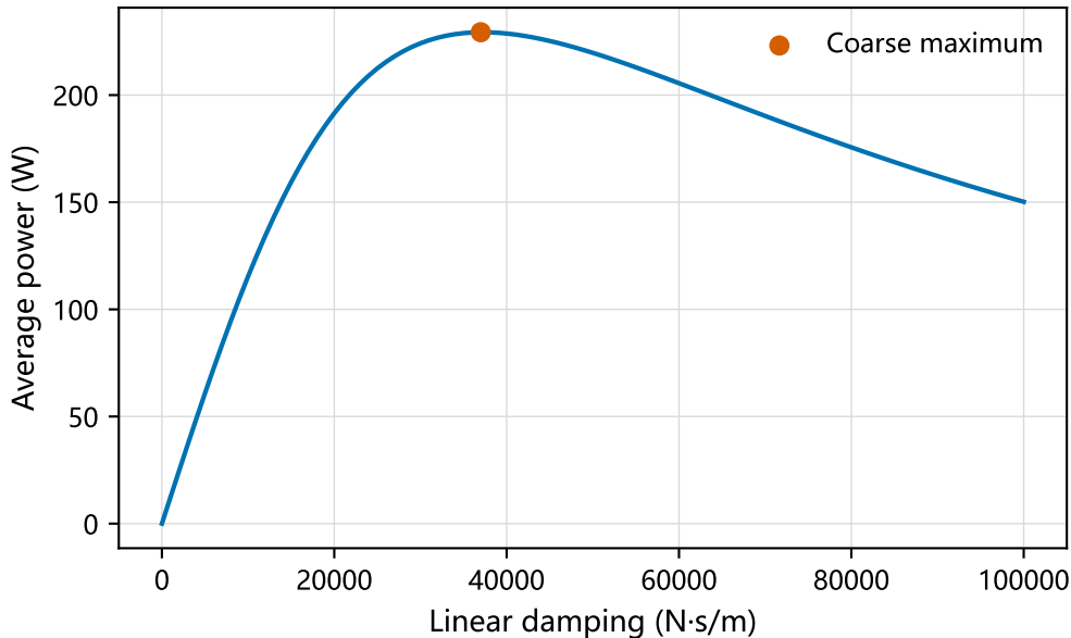
Q2 constant-damping power curve
