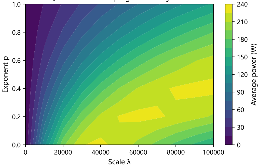
Q2 nonlinear-damping coarse objective
