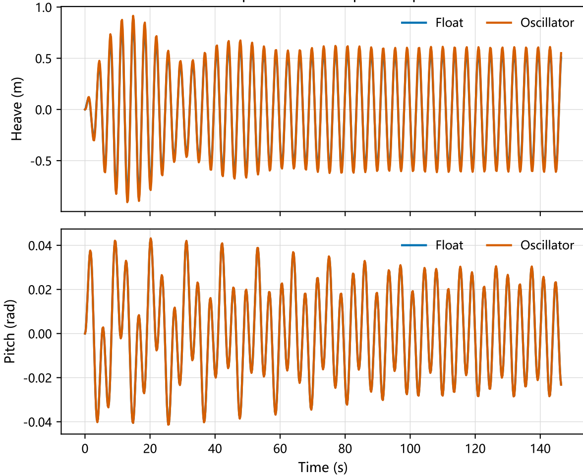
Q3 coupled heave and pitch response
