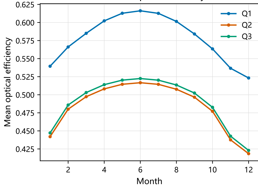
Seasonal optical efficiency
