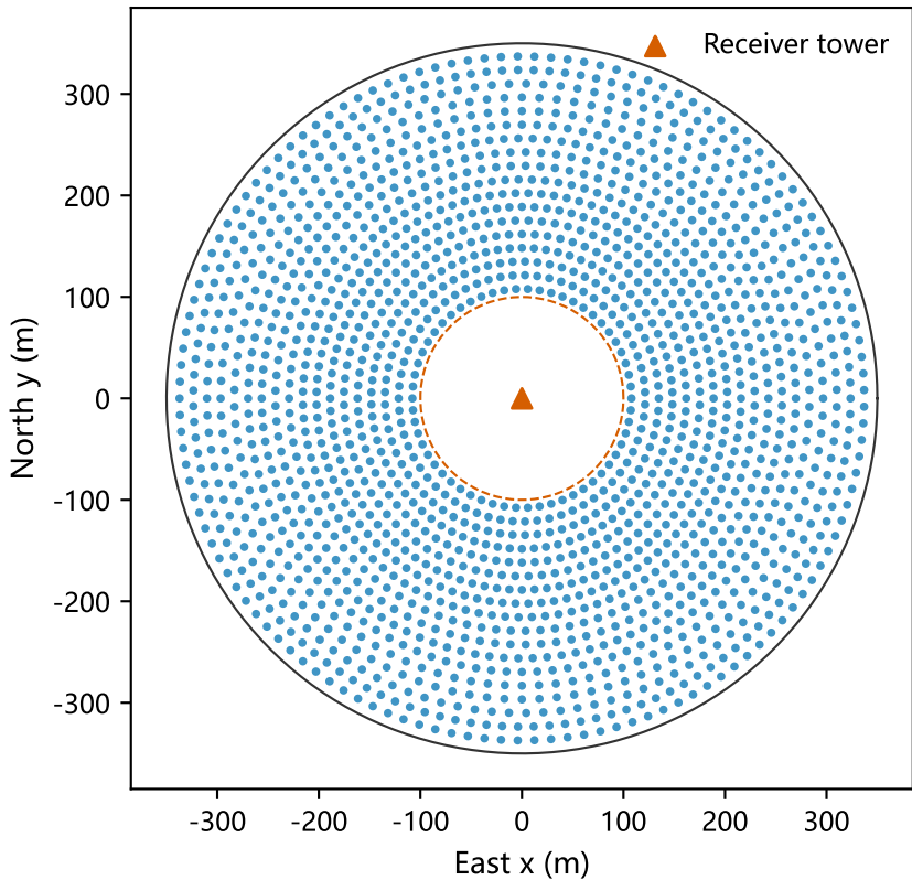
Q1 official heliostat field (1745 mirrors)
