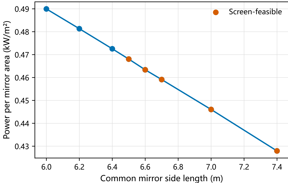
Q2 size slice and rated-power boundary
