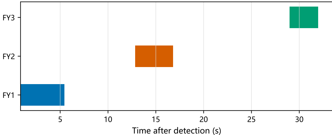
Q4 three-UAV obscuration intervals
