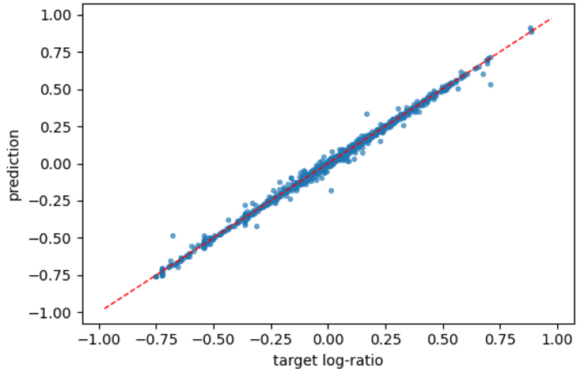
Spearman(active)=0.9946
