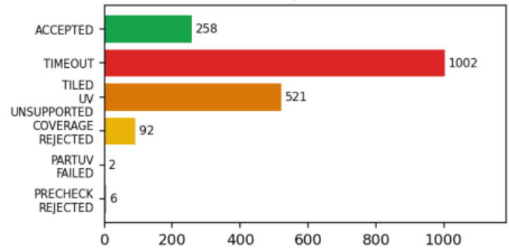
Build funnel (attempted 1881, acc 13.7%)
