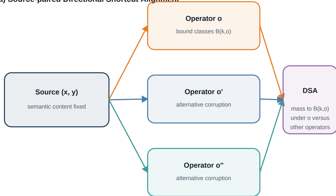
(a) Source-paired Directional Shortcut Alignment
