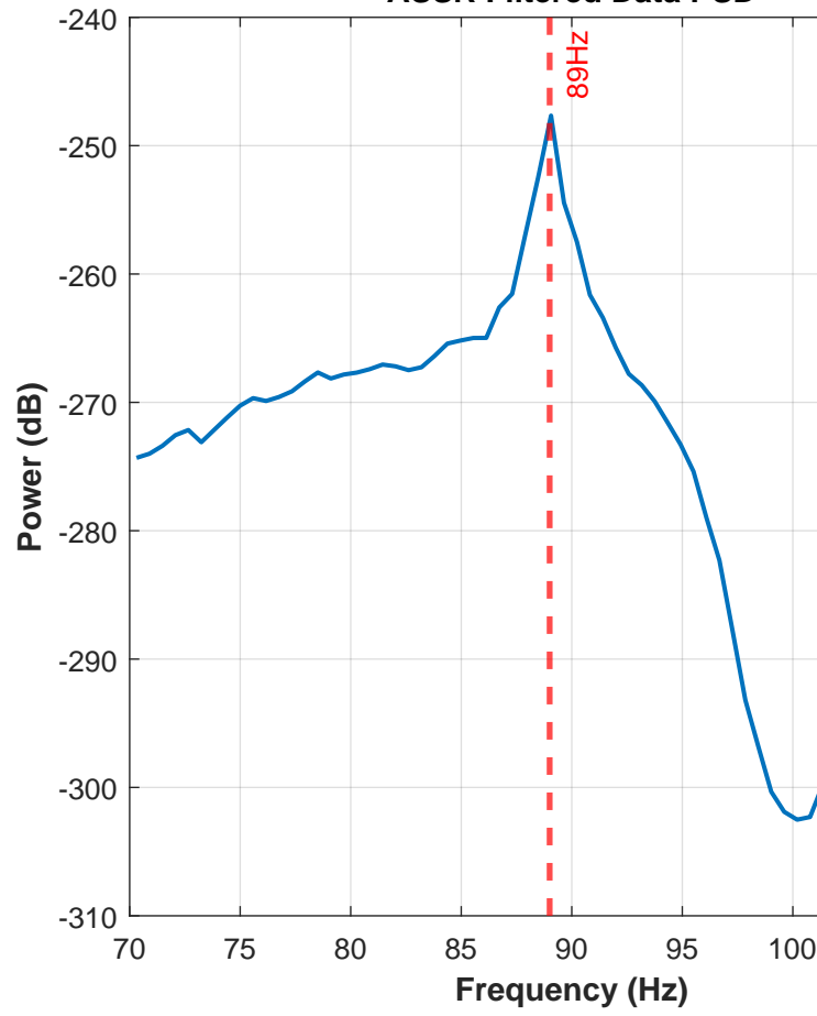
ASSR Filtered Data PSD
