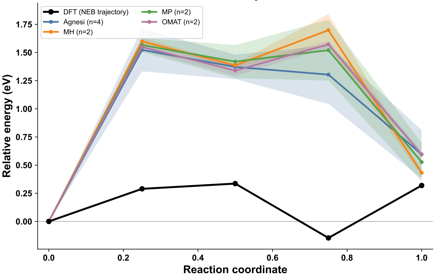
Path 1–4: model-family mean \pm 1 SD
