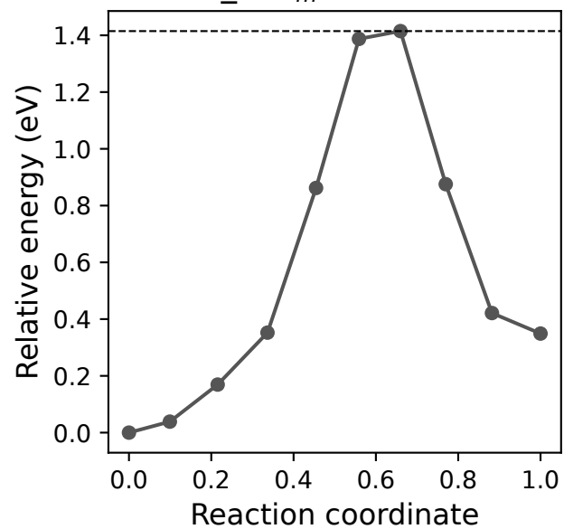
(f) neb_5: E_m = 1.415 eV
