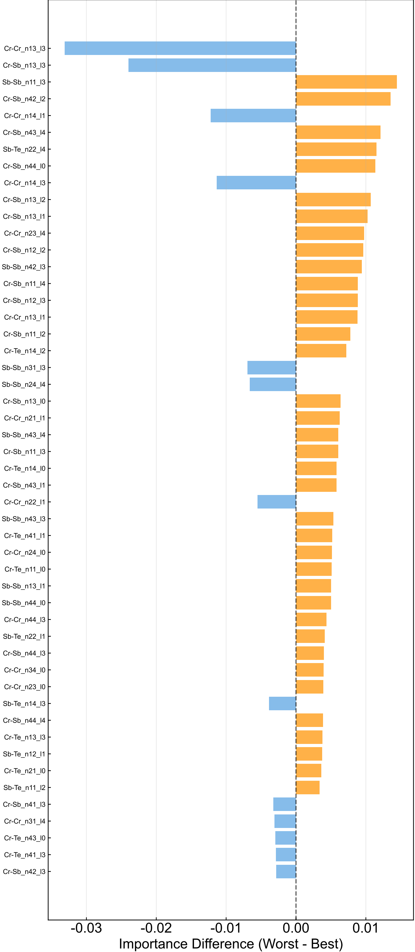
Features Differentiating Model Performance (Top 50)
