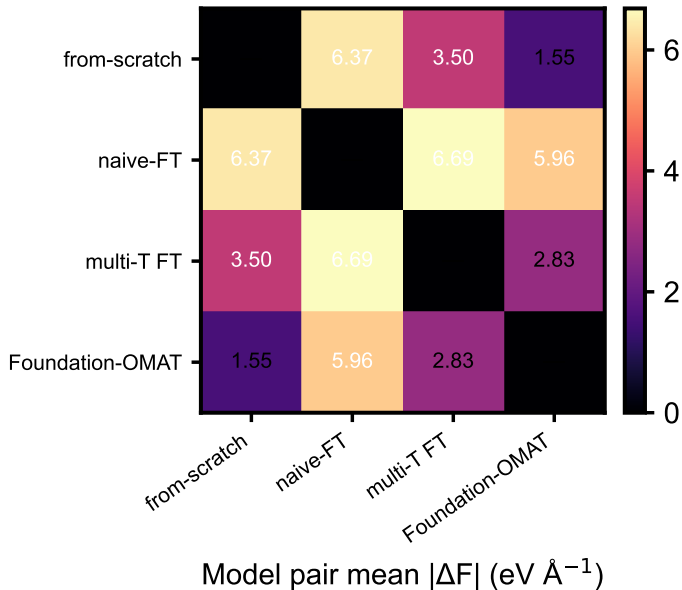
Force disagreement at step 462,200
