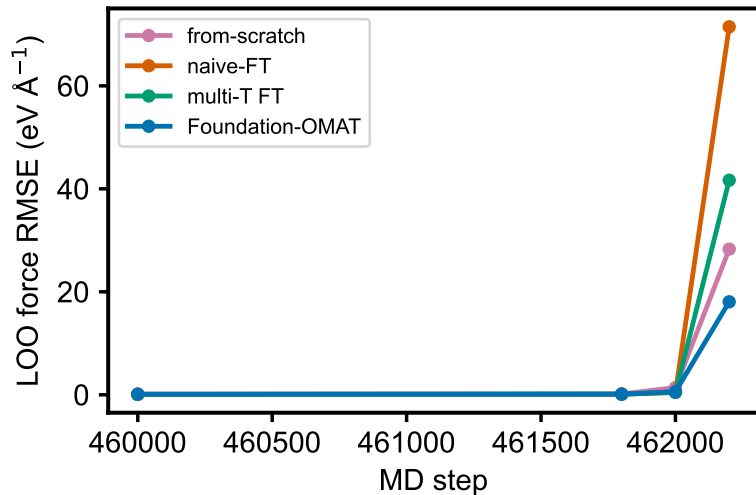
Model-to-other-model disagreement
