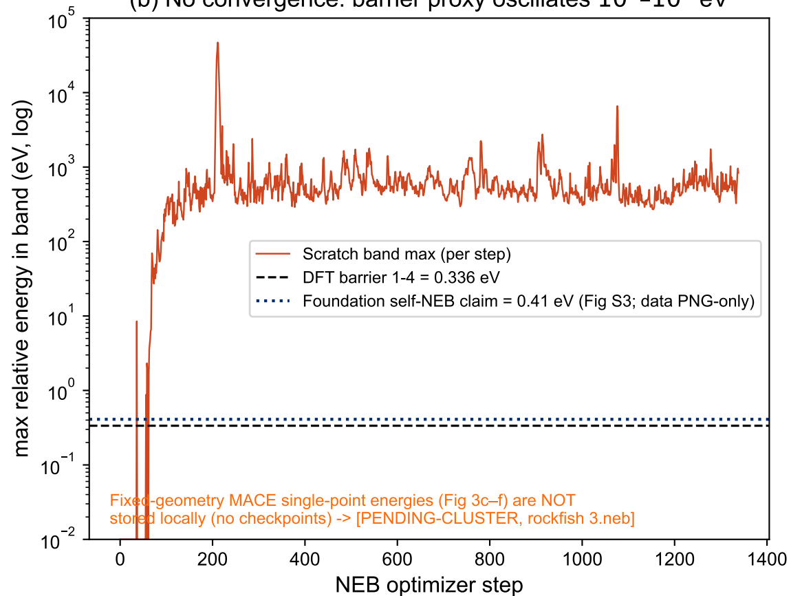
(b) No convergence: barrier proxy oscillates 10^2 - 10^4 eV
