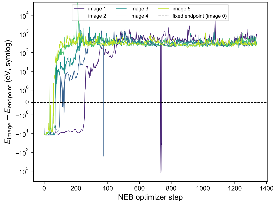
(a) Scratch self-NEB trajectory (neb_optm_1-scratch.xyz)
