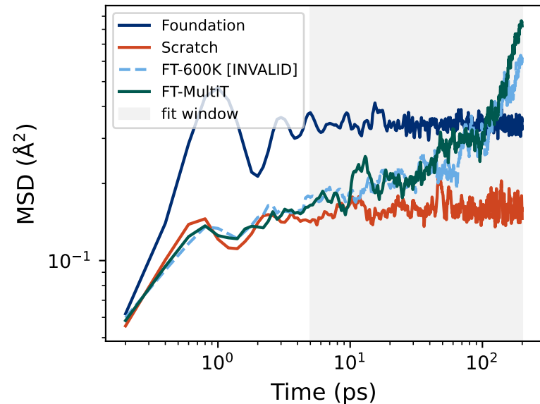
(a) Mean Squared Displacement
