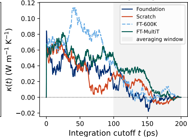
(b) Green-Kubo Running Integral \kappa(t)
