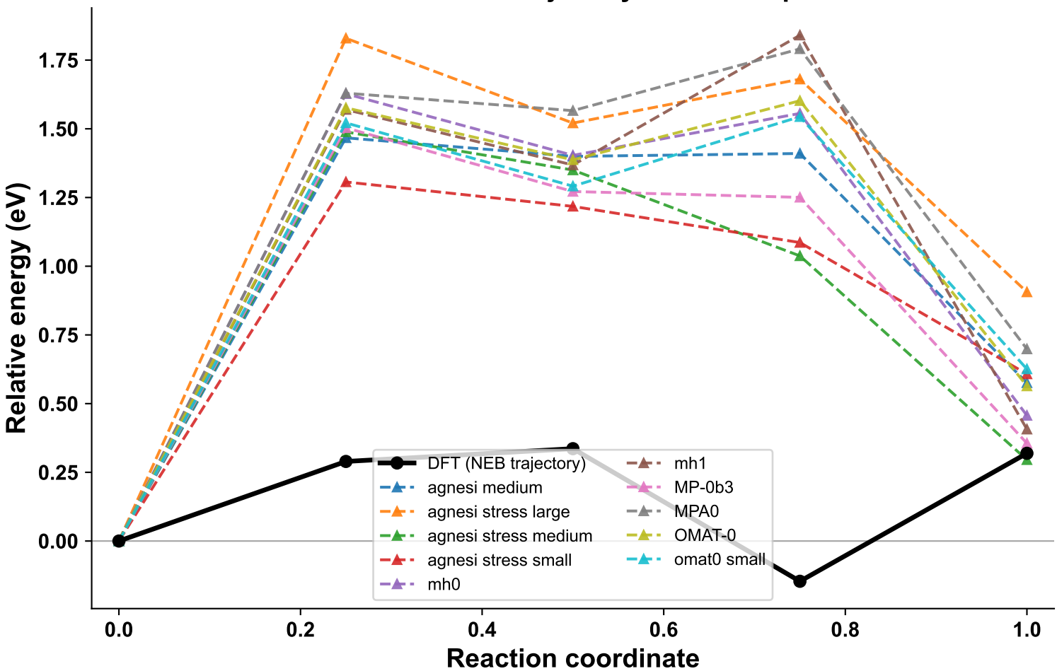
Path 1-4: DFT NEB trajectory and MACE profiles
