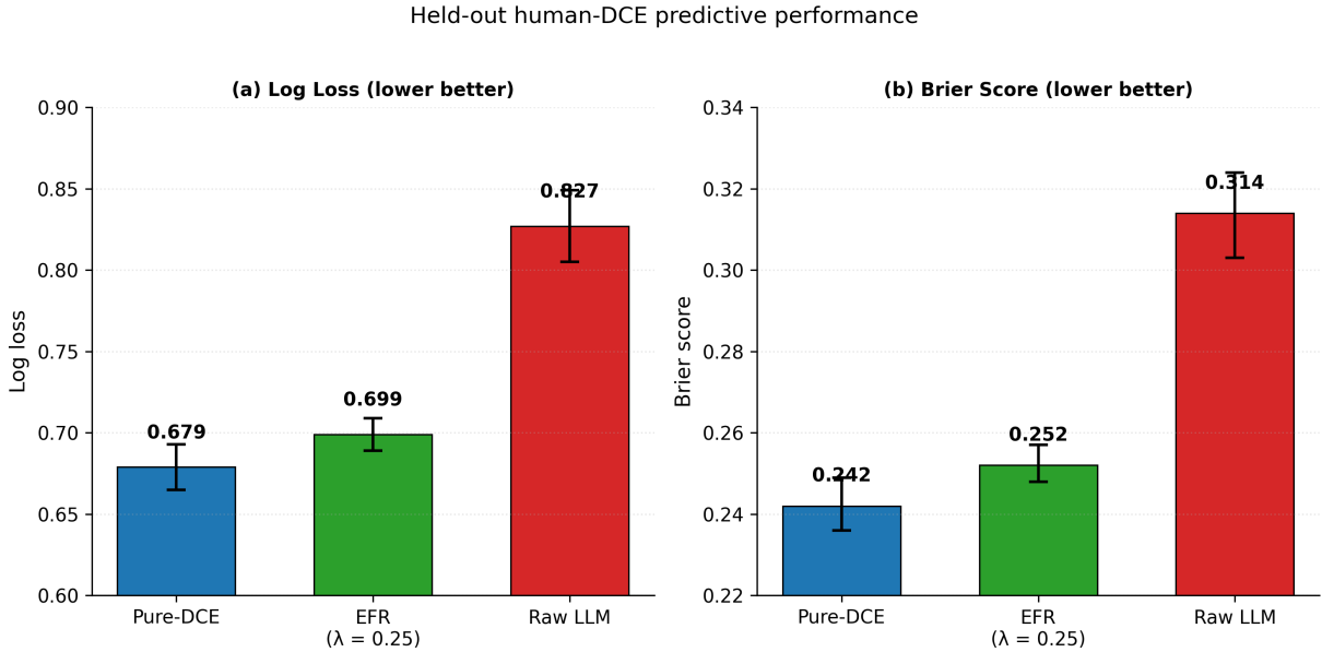
Figure 1: Held-out human-DCE predictive performance on the N = 813 alternative-level binary-outcome rows from the N = 205 held-out respondents (each row is one of three alternatives within one of six tasks), with respondent-cluster bootstrap 95% confidence intervals (2,000 replicates). (a) Log loss; (b) Brier score. EFR does not outperform the Pure-DCE endpoint; it recovers much of its predictive discipline (EFR log loss 0.699 vs. Pure-DCE 0.679, \Delta = 0.020 ) while retaining a nonzero narrative component permitted inside the convex blend with P_{\text{emp}} . The Raw LLM endpoint is materially worse on both metrics (log loss 0.827, Brier 0.314).
