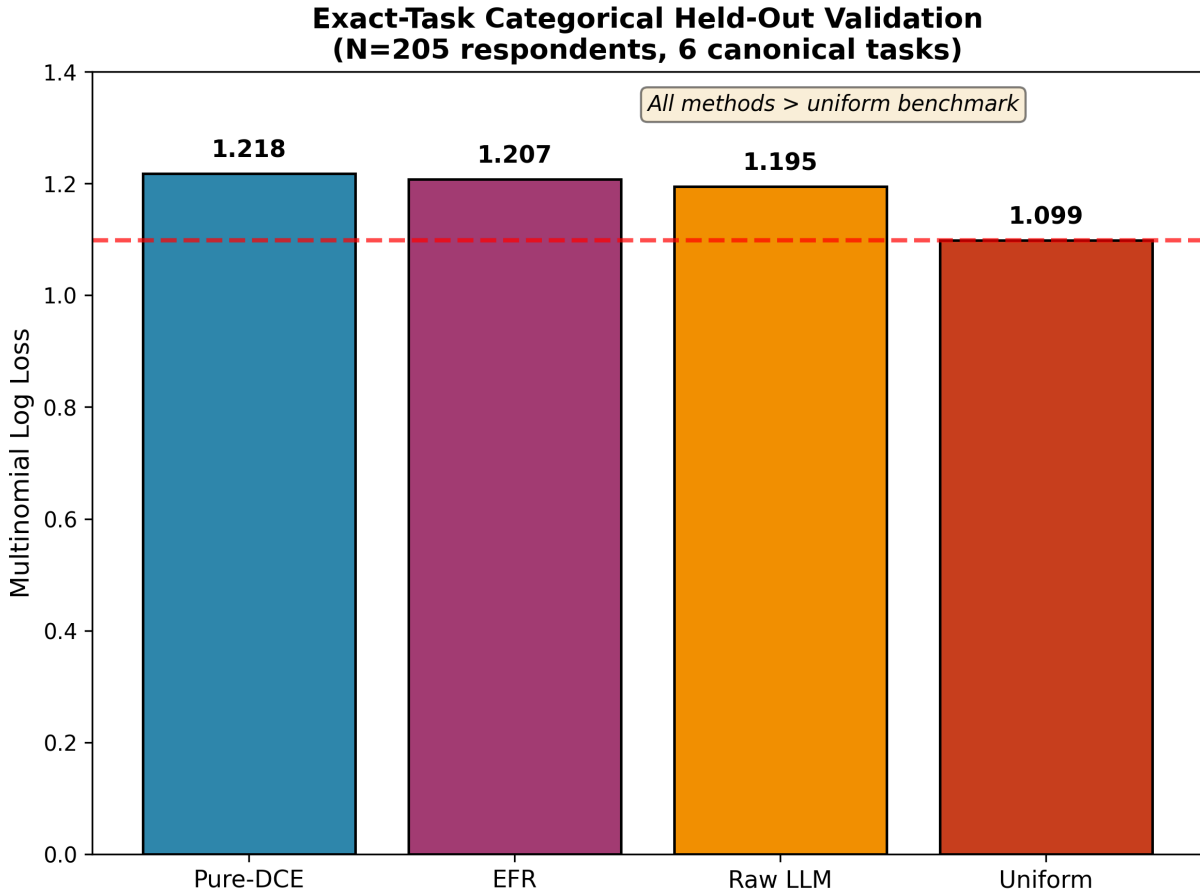
Figure 1: Exact-task categorical held-out validation on the six canonical DCE tasks ( N = 205 held-out respondents, 1,230 respondent-task observations). Multinomial log loss for Pure-DCE (1.218), EFR (1.207), Raw LLM (1.195), and the uniform-probability benchmark ( \log(3) = 1.099 ). All three model-based approaches exceeded the uniform benchmark; EFR did not improve exact-task predictive performance relative to Raw LLM ( \Delta = 0.013 ) and did not outperform the equal-probability benchmark. This negative result is reported transparently; the paper’s primary contribution is structural regularization and behavioral constraint, not predictive superiority.
