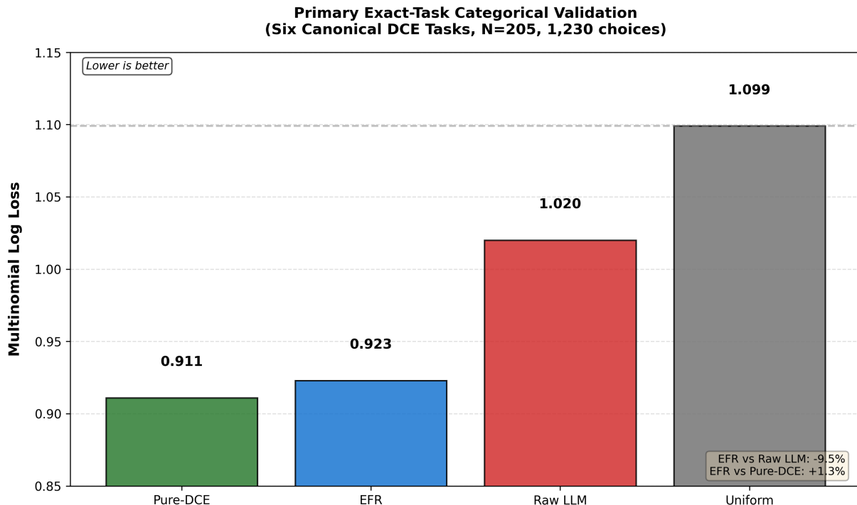
Figure 1: Held-out-respondent validation multinomial log loss on the six administered DCE choice tasks (Pure-DCE: 0.911; EFR: 0.923; Raw LLM: 1.020; uniform benchmark: 1.099; N = 205 held-out respondents, 1,230 choices). Because all respondents completed identical tasks, this validation evaluates generalization to unseen respondents rather than to unseen choice tasks or attribute profiles.
