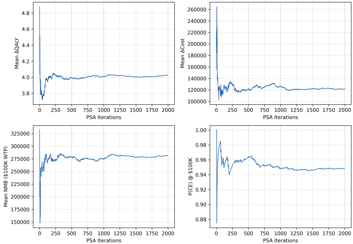
Figure S6: PSA convergence across iteration counts (2,000 structurally valid iterations, 0 structural rejections, seed = 42). Cumulative means of \Delta QALY , \Delta Cost , NMB, and P(CE) . Vertical dotted lines at 500, 1,000, and 2,000 iterations. Estimates stable from ~500 iterations.
