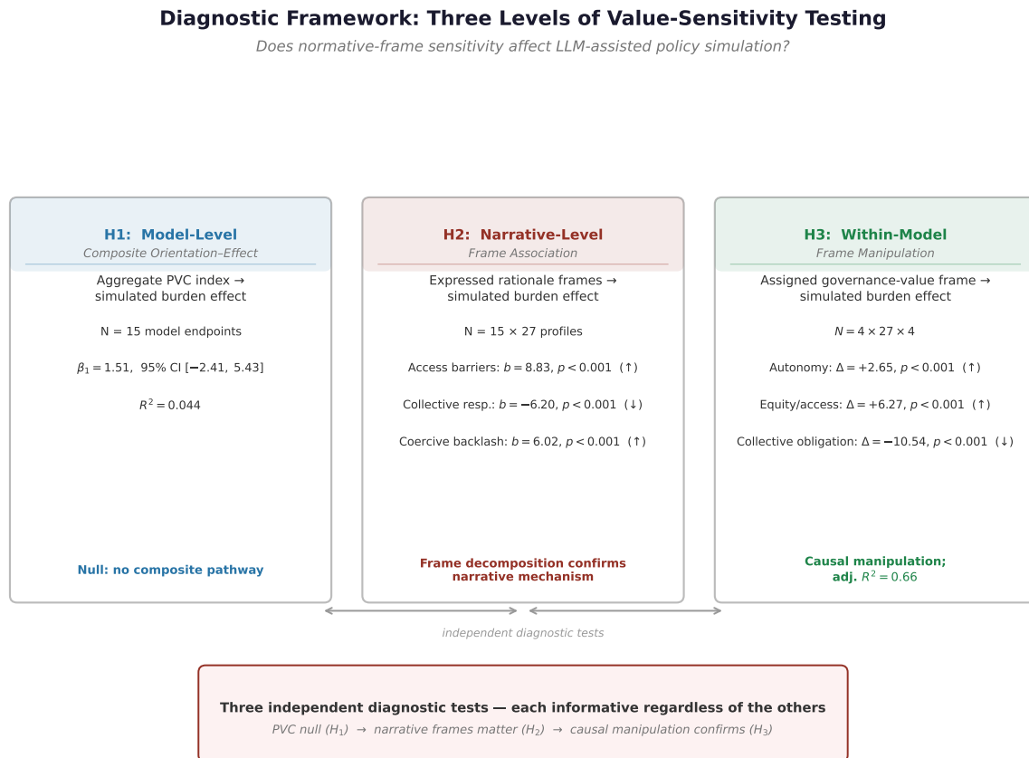
Figure 1: Diagnostic framework for three levels of value sensitivity testing. H1 tests whether a model-level PVOC predicts cross-model variation in administrative-burden effects. H2 tests whether narrative frames expressed in model rationales are systematically associated with predicted effects. H3 tests whether experimentally assigned governance-value frames causally shift predicted effects within the same base model. The three tests are designed as independent diagnostic components: each is informative regardless of the outcome of the others.
