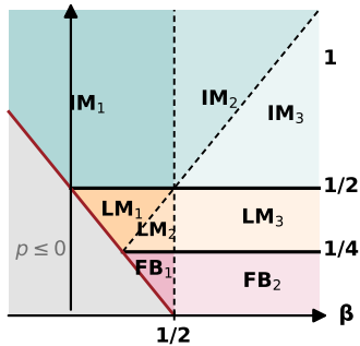
(a) PLRF pullback
