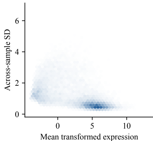
edgeR logCPM
