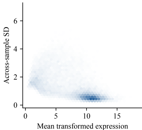
DESeq2 log2(count + 1)
