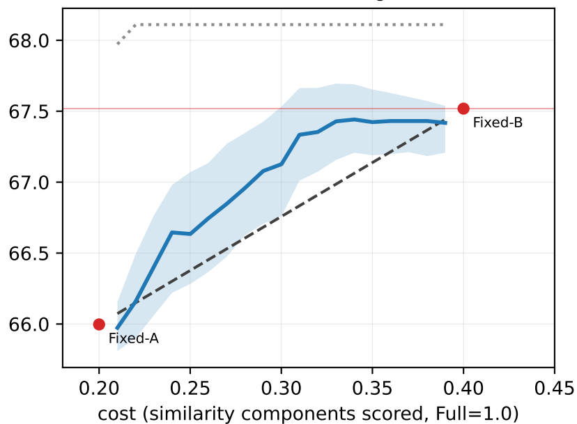
MSR-VTT (IV2) noASR sd(gain)=11.2
