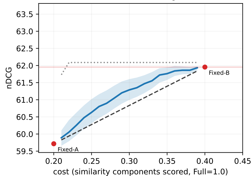
MSR-VTT (mCLIP) ASR sd(gain)=9.8
