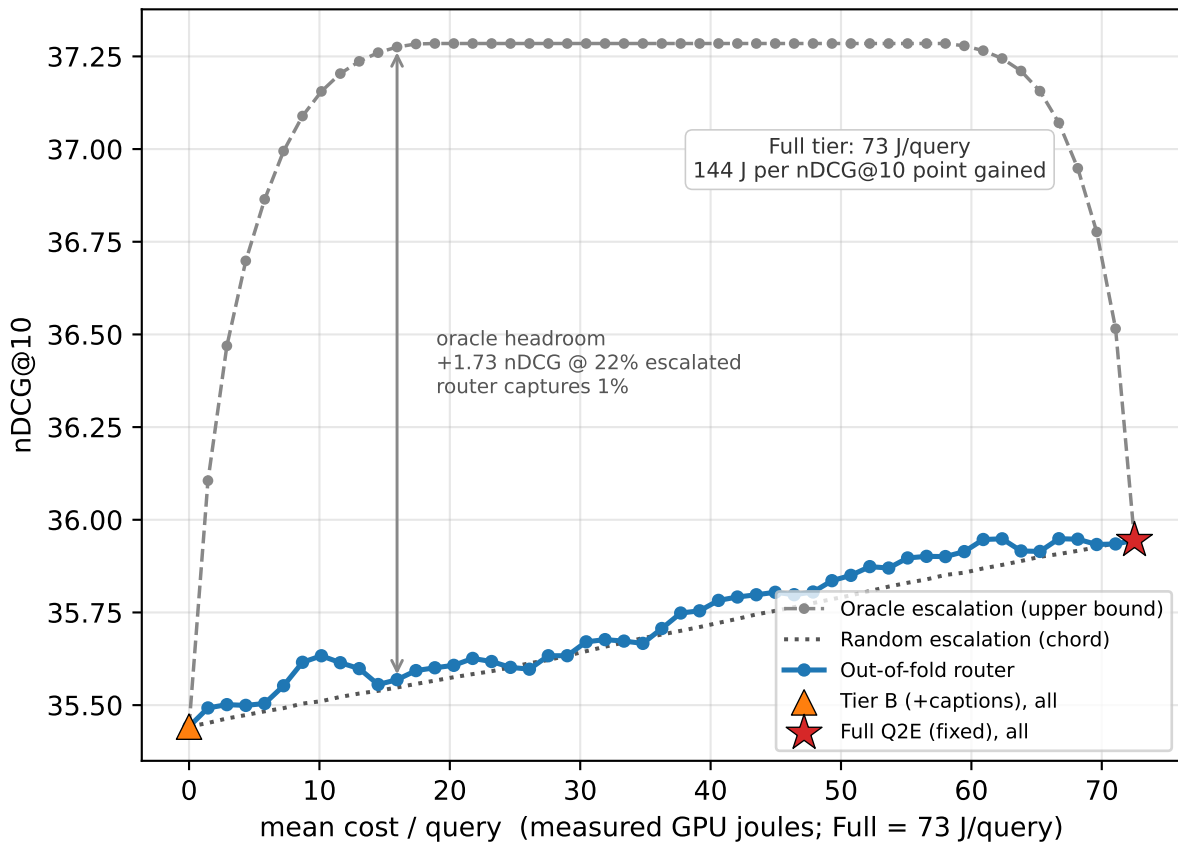
The Full event tier is dominated on the energy frontier (MultiVENT 2.0 test queries; qwen2.5:3b decomposer on GPU1)
