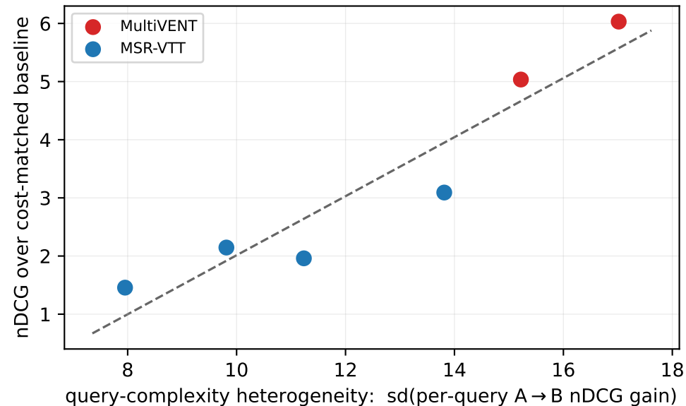
Oracle headroom Spearman rho = +0.94 (n=6 cells)
