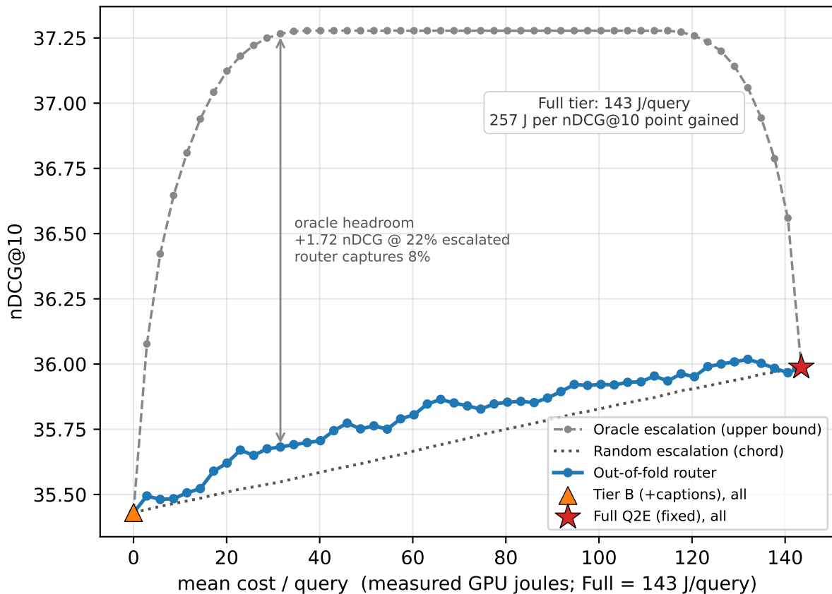
The Full event tier is dominated on the energy frontier (MultiVENT 2.0, 2,544 test queries; qwen2.5:7b on GPU1)
