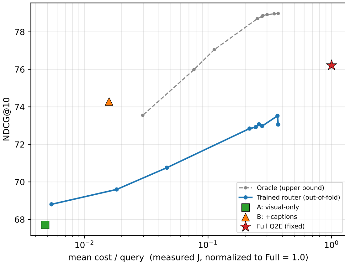
MultiVENT / MultiCLIP (noASR) (n=259, 9.24 gold/query)
