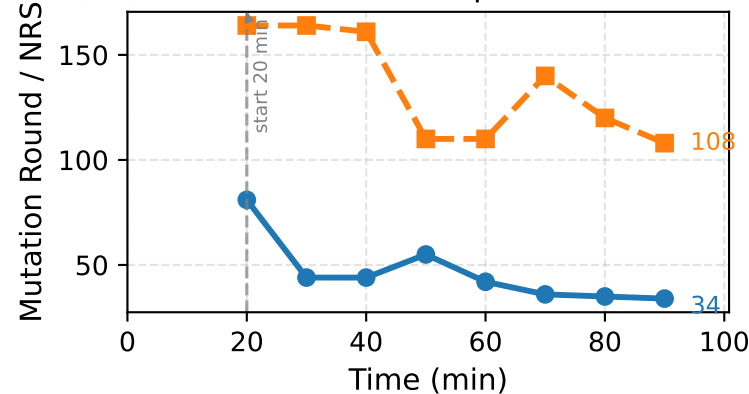
(c3) Smart Camera — Exploration Efficiency
