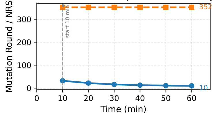
(a3) YLDP05YL — Exploration Efficiency
