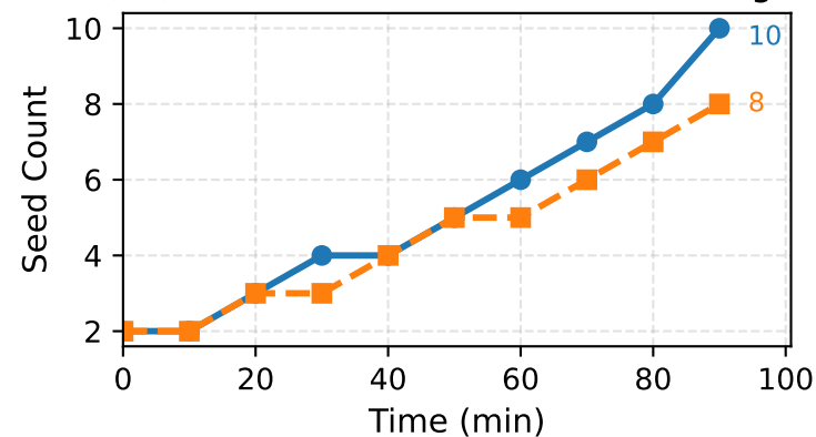
(c1) Smart Camera — Seed Pool Length
