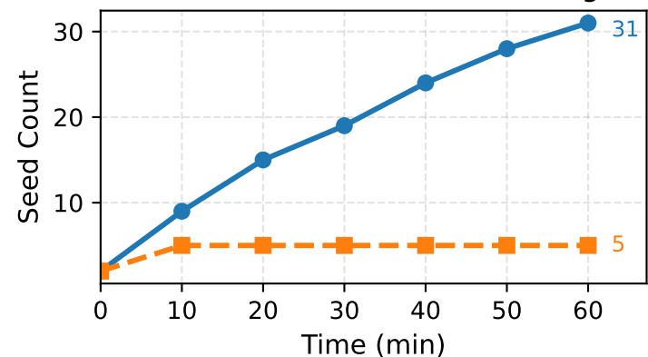
(a1) YLDP05YL — Seed Pool Length
