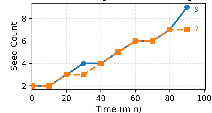
(b1) Smart Plug — Seed Pool Length
