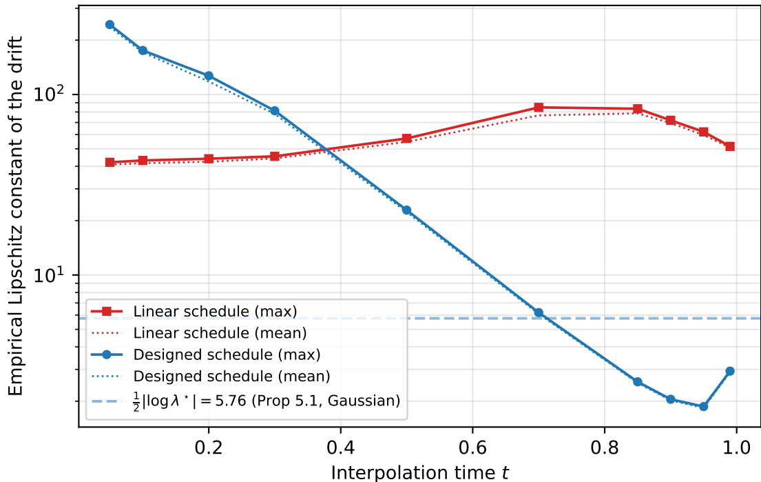
NS 128×128, white-noise prior, learned drift: linear vs designed schedule
