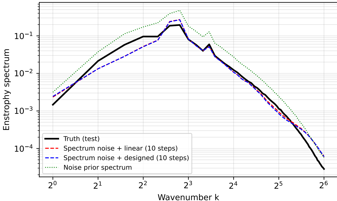
NS 128x128: spectrum noise prior, \lambda^* = 4.988e-01
