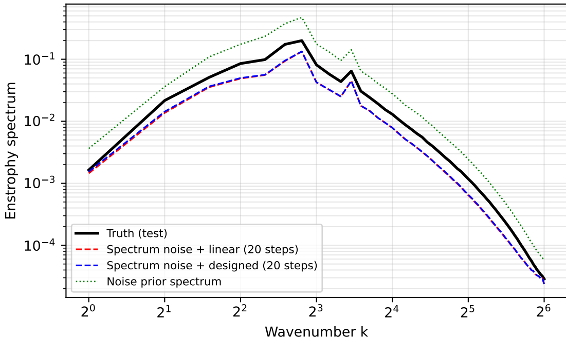
NS 128x128: spectrum noise prior, \lambda^* = 5.064e-01
