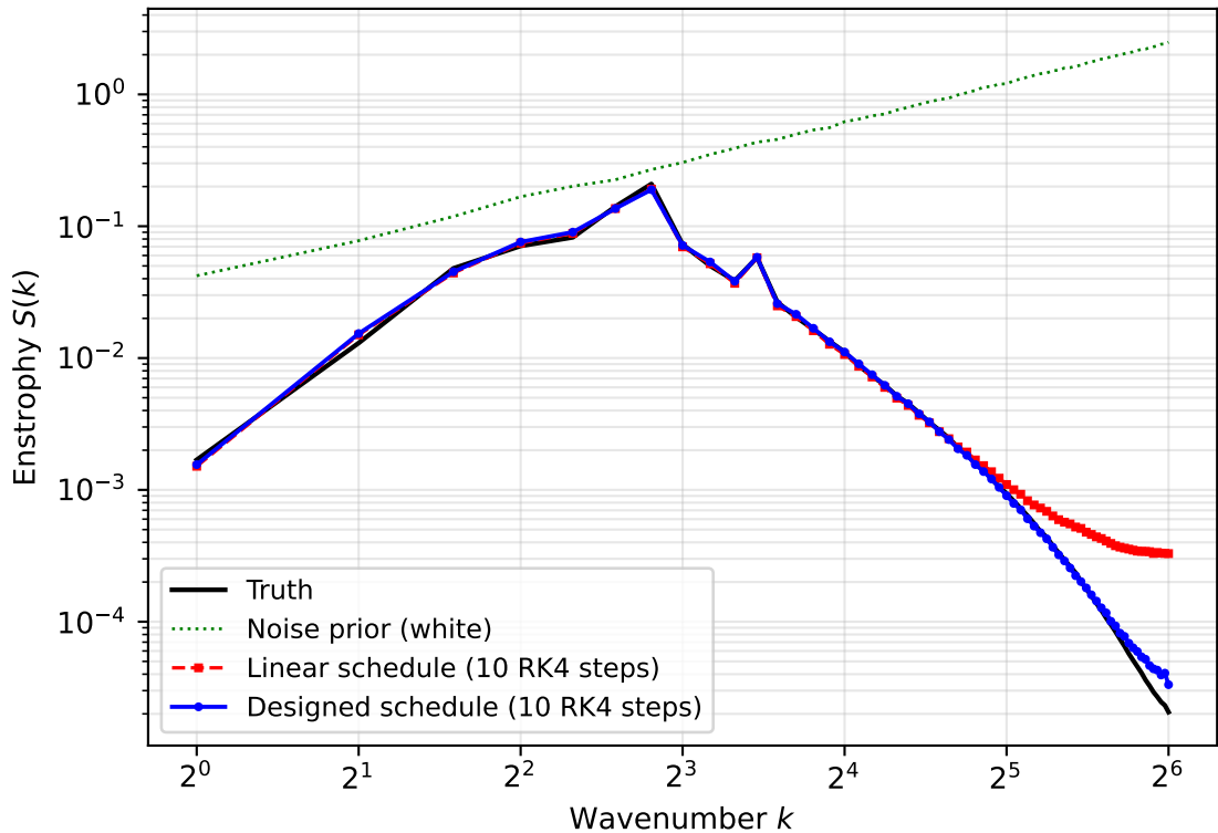
NS 128×128, white-noise prior: linear vs. designed schedule
