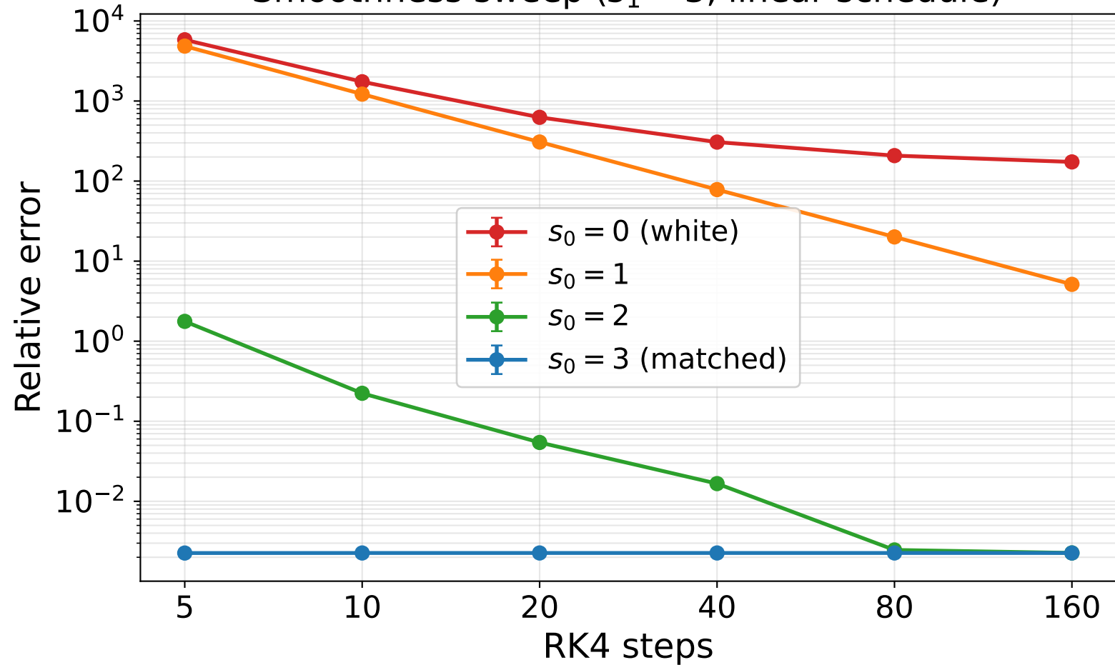
Smoothness sweep ( s_1 = 3 , linear schedule)
