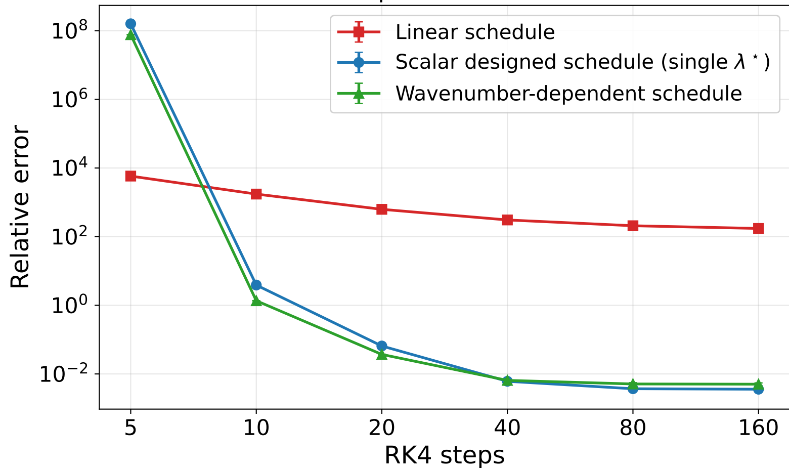
Wavenumber-dependent vs scalar schedule
